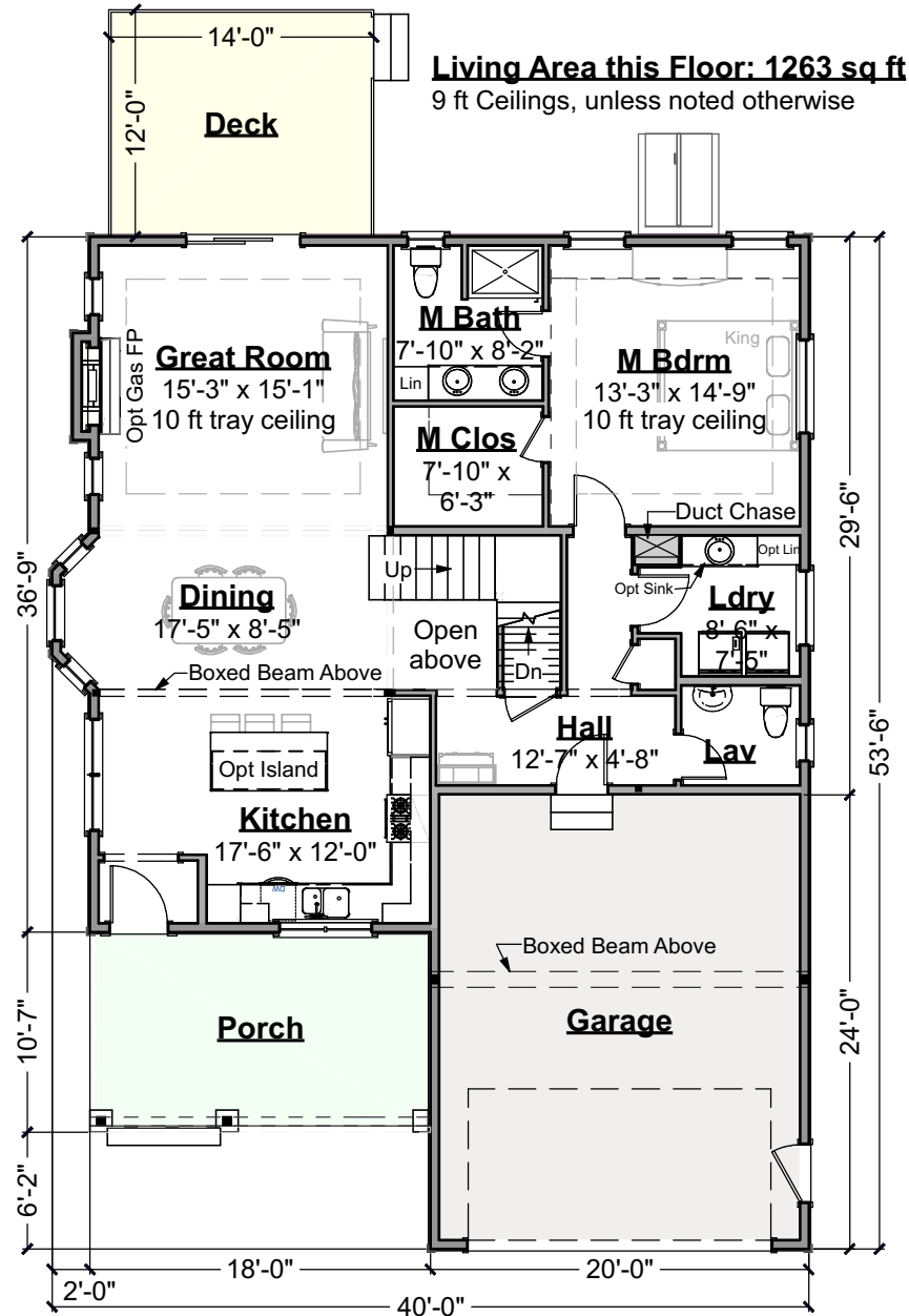
First Floor Plan Scale: 3/32" = 1'-0"
